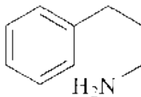
Primary amine (basic)
