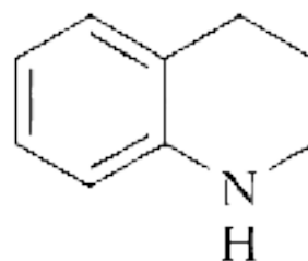
Secondary amine (basic)
