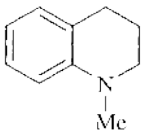
Tertiary amine (basic)
